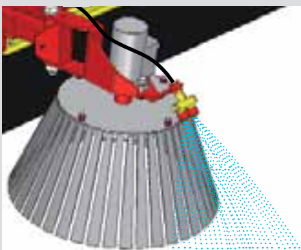
SPRIKLING KIT FOR SIDE BRUSH
